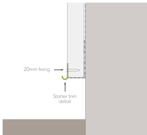
Fig. 17b - Starter trim detail
