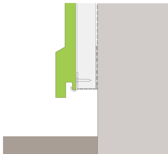
Fig. 18 - First board install
