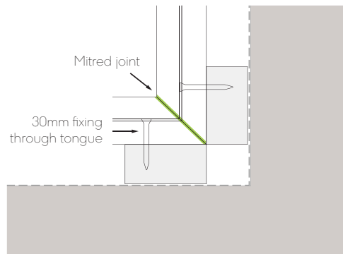
Fig. 9 - Internal mitred corner detail
